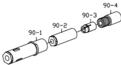
MCS-50250LBK-90G Lock Bolt Assy 3/16" Multi-Grip
