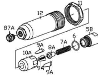
MCS-50250LBK-90B Rivet Head Assy 5/16"
