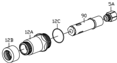
MCS-50250LBK-90E Lock Bolt Assy 1/8", 5/32"
