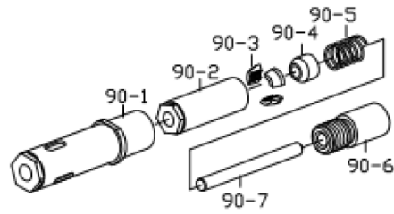
MCS-50250LBK-90D Lock Bolt Assy 1/4" BOM
