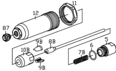
MCS-50250LBK-90C Rivet Head Assy 1/8", 5/32"
