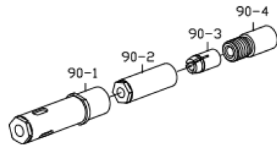
MCS-50250LBK-90H Lock Bolt Assy 1/4" Fixed-Grip
