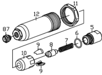
MCS-50250LBK-90A Rivet Head Assy 3/16", 1/4"
