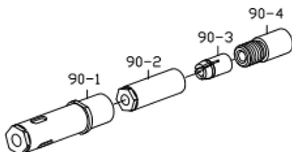
MCS-50250LBK-90I Lock Bolt Assy 1/4" Multi-Grip
